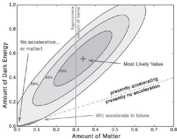
Figure 1. This is a reproduction of figure 2 from the new research paper with annotations added. The contours encircle the values of the matter density and dark energy (in the form of a cosmological constant) that best fit the supernova data (in units of the critical density of the universe). The contours show one, two, and three standard deviations. The best fit is marked by a cross. The amount of matter measured by other observations lies approximately around the orange line. The contours lie almost entirely in the accelerating region, and the tiny patch that is not yet accelerating will nevertheless accelerate in the future.
