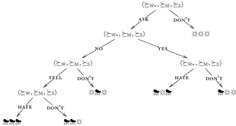
Figure 4: The description tree t \mapsto S(t, \mathbb{M}) = S_{\mathbb{M}}(t, \emptyset) of Mary's beliefs. This is also the description tree of S_{M^W} and S_{M^{WW}} .
